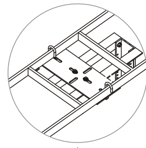
Rack Ladder Mounting Kit
