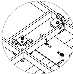
Corner Clamp Kit
