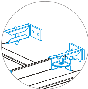
Wall Bracket Kit
